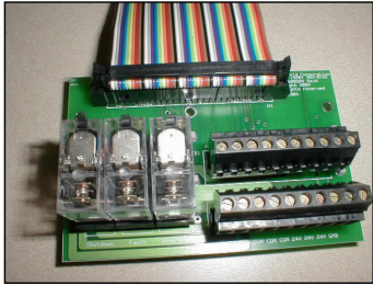
PCB and Cable Assembly
